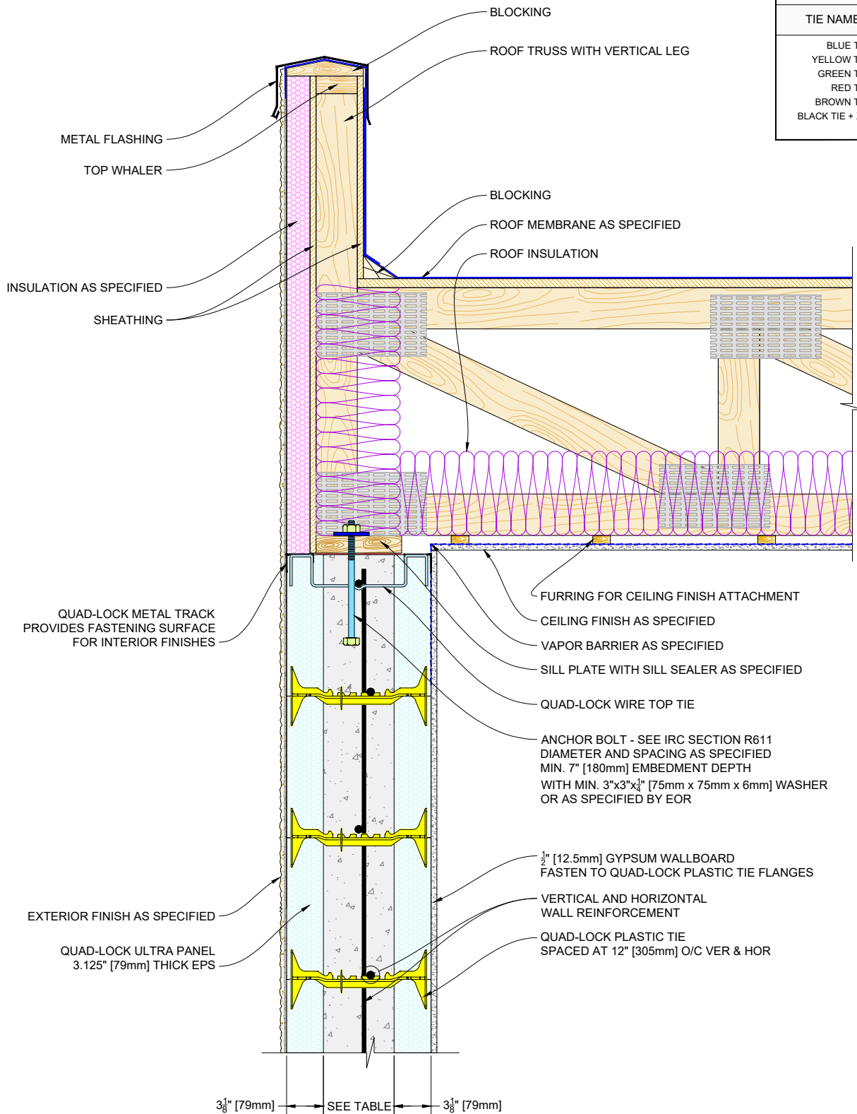
QUAD-LOCK R-28 [U-0.21] WALL
